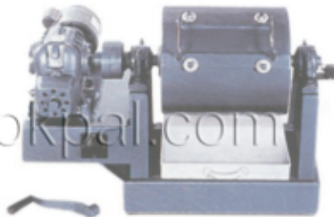
Los Angeles Abrasion Testing Machine
